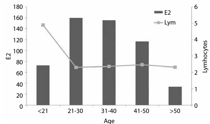
Figure 1. Median estradiol (E2) and lymphocyte levels in terms of age-dependent groups.
